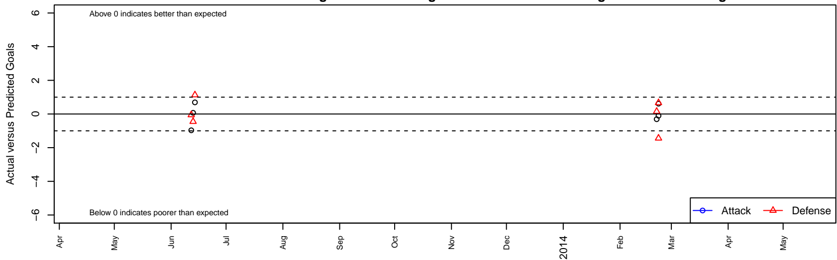
CCV Stars Orange B96 Dots are actual minus expected GF (blue circles) and GA (red triangles). Blue line is smoothed change in attack strength. Red is smoothed change in defense strength.
